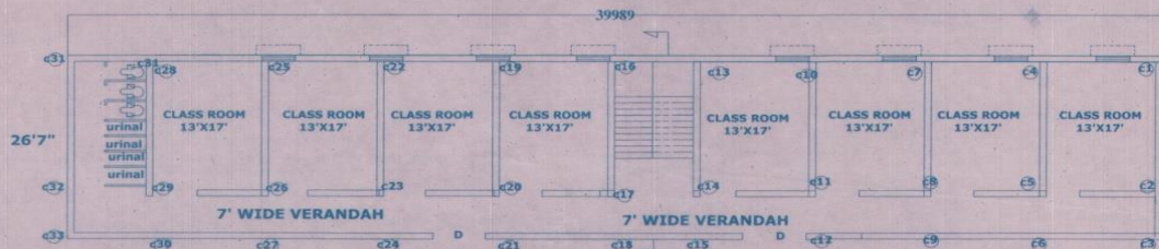
2ND FLOOR PLAN (PROP.)
