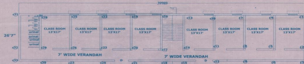
3RD FLOOR PLAN (PROP.)
